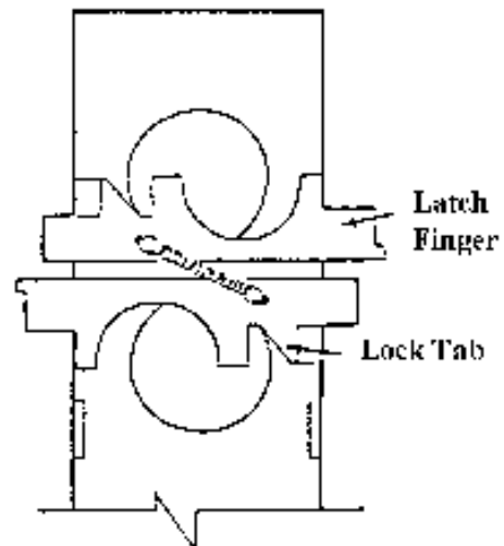
Fig. 14 Rear Spacer
